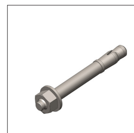
segmented anchors Hilti HST2 M12 x 115/20
