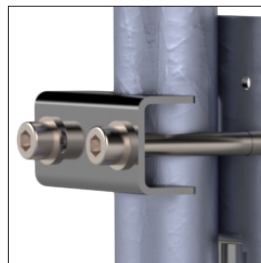
AT241 002 stainless steel clamp on pipe
